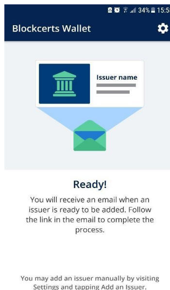
Figure 8 Final Screen
